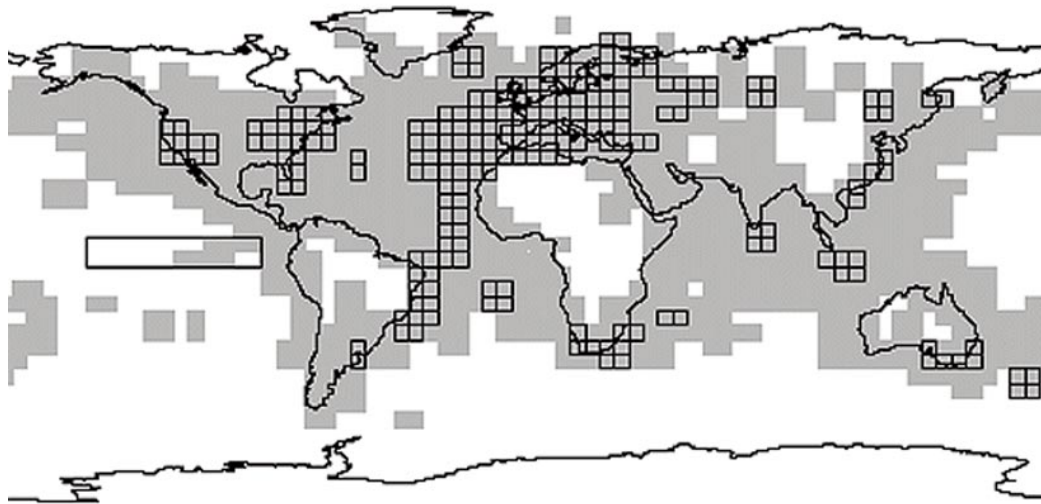
Figure 2. Distribution of the (1082) nearly continuous available monthly land air-sea surface temperature gridpoint data available from 1902 onward indicated by shading. The squares indicate the subset of 219 grid points with nearly continuous records extending back to 1854 that are used for verification. Northern Hemisphere (NH) and global (GLB) mean temperature are estimated as areally weighted (i.e., cosine latitude) averages over the Northern Hemisphere and global domains, respectively. The large rectangle indicates the tropical Pacific SST subdomain discussed in the text. The small rectangle in the eastern tropical Pacific shows the traditional Niño-3 region. These data are described in more detail by Jones (Jones, 1994). [Initial comparisons using an updated version of this dataset (e.g., Jones et al., 1999) showed no significant differences in the large-scale structure of the twentieth century surface temperature dataset, although some specific differences are notable, particularly during the World War II years (e.g., the mid-1940s). Future updates of these reconstructions will employ this latter instrumental surface temperature dataset.] [Reprinted with permission from Mann et al. (Mann et al. 1998).]
